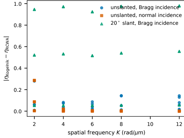
Fig. S4. Absolute deviation of Kogelnik first-order efficiency from RCWA over the 90-case grid, one series per geometry.
