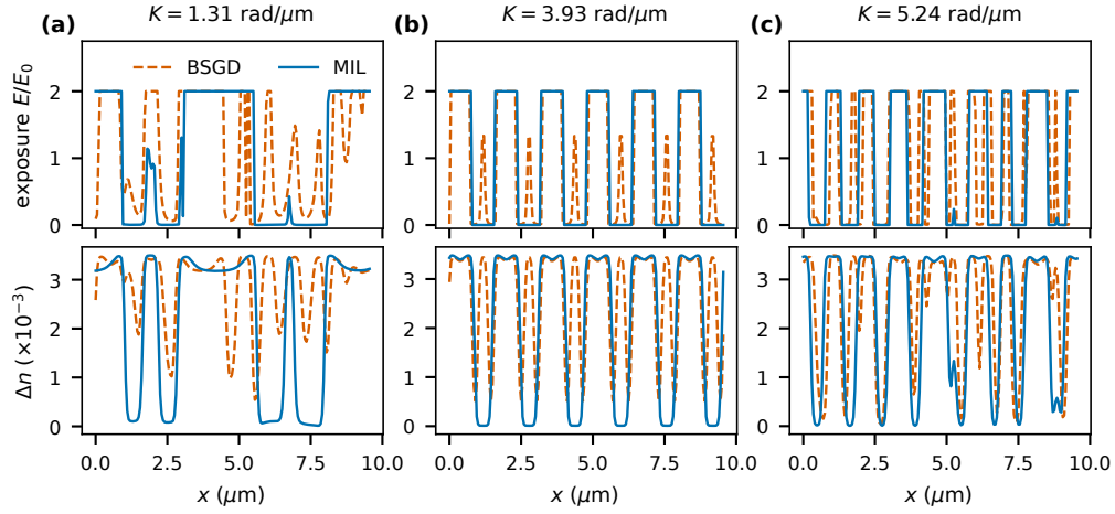
Fig. S1. Exposure E/E_0 (top) and recorded \Delta n (bottom) for BSGD and MIL, same K , budget B_c = 2 , seed and 9.6 \mu\text{m} section as Fig. 2.
